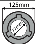
Tank Neck Triple bayonet with Internal flange
